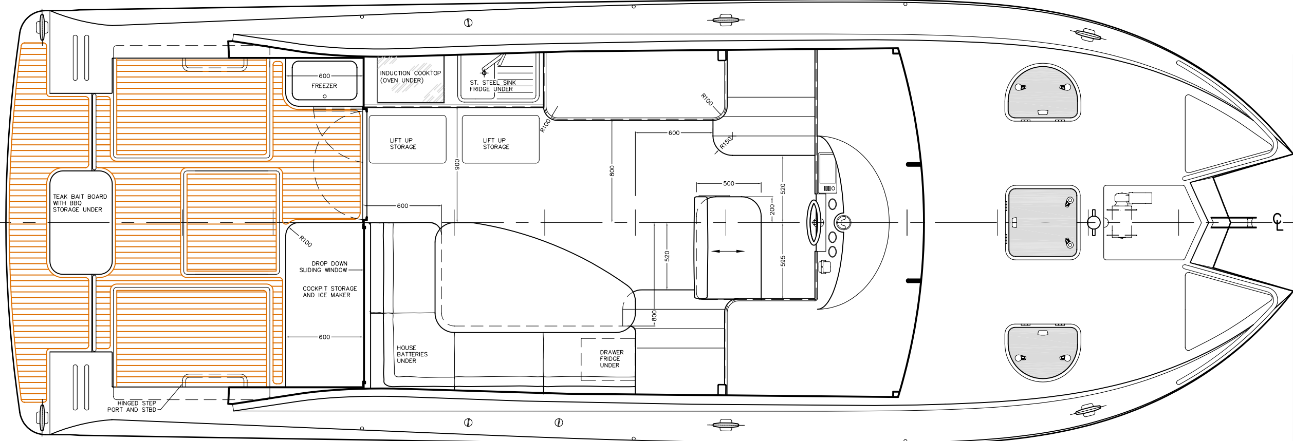
MAIN DECK LAYOUT
