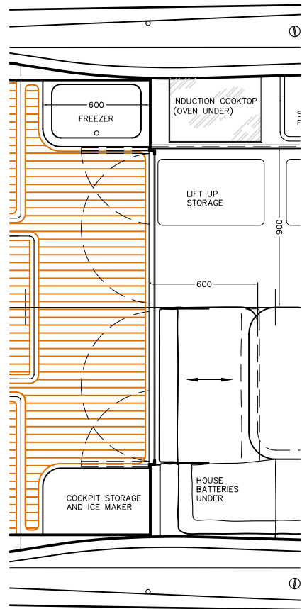
ALTERNATE AFT DOOR DETAIL
