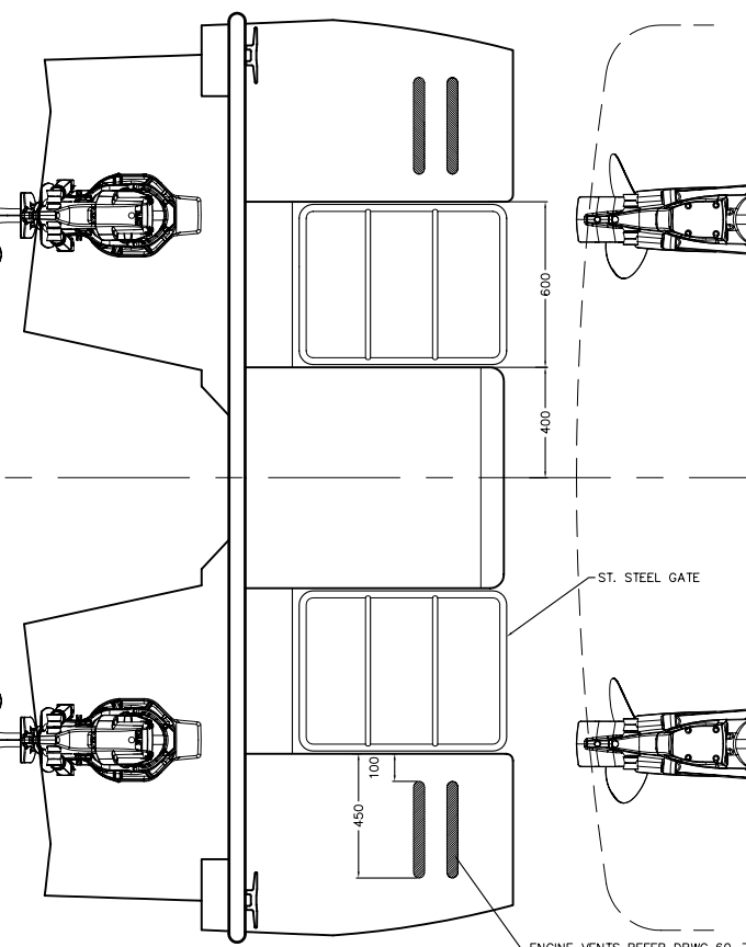
TRANSOM DETAIL
