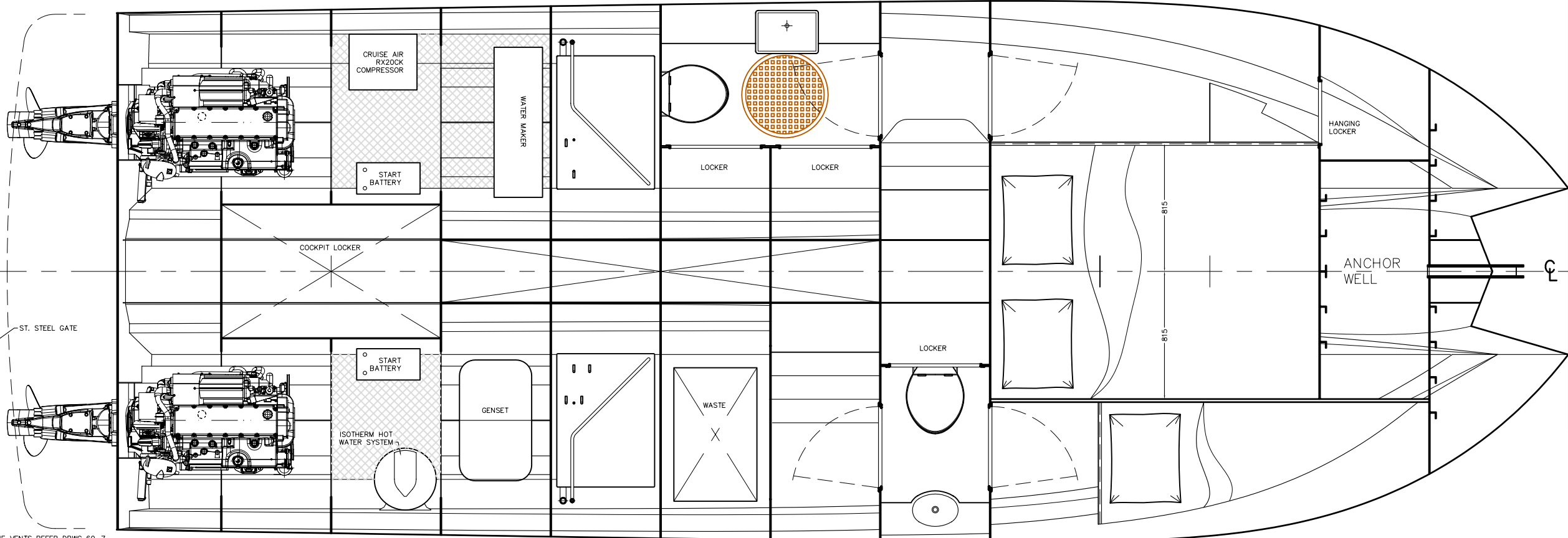
LOWER DECK LAYOUT
