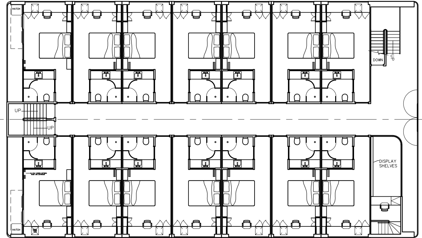
MAIN DECK
