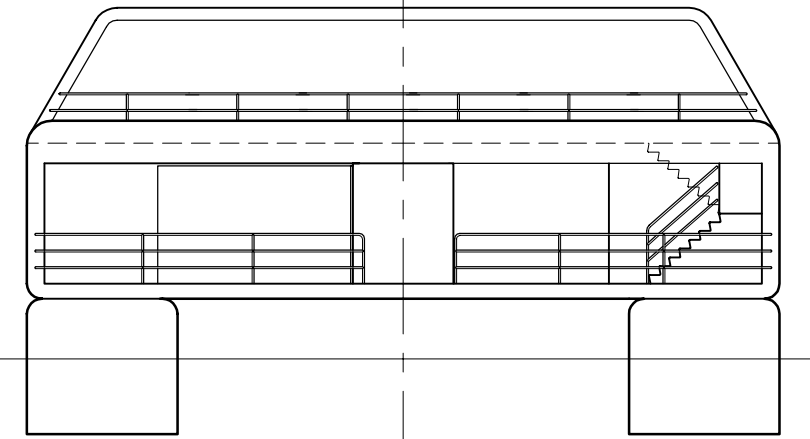
BOW
